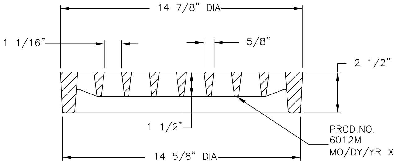
GRATE SECTION
